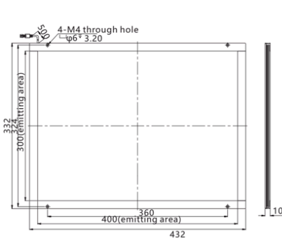
LS-2PFS400300
