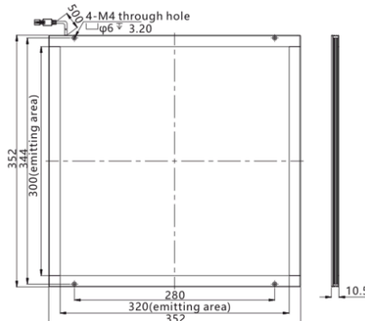
LS-2PFS320320
