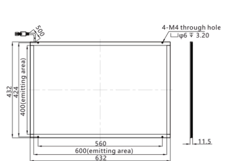
LS-2PFS600400
