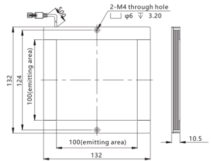
LS-2PFS250200
