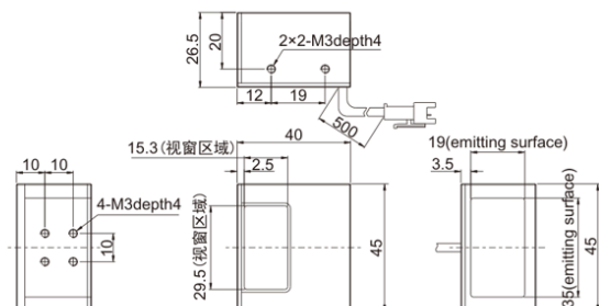
5.LS-2COXR60
