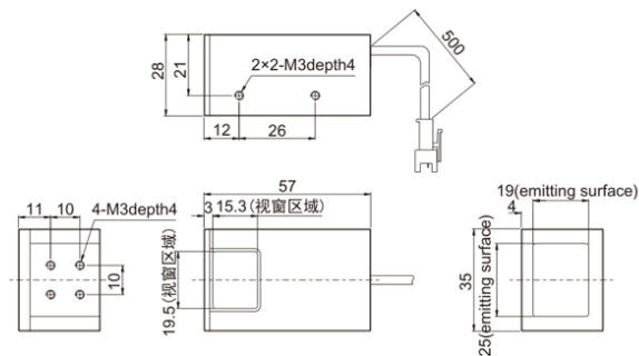
3.LS-COXR3520
