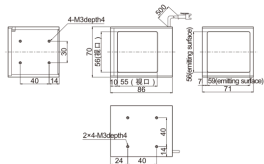
5.LS-2COXR60
