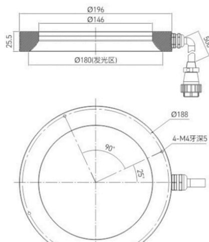
LS-HRM196-8
