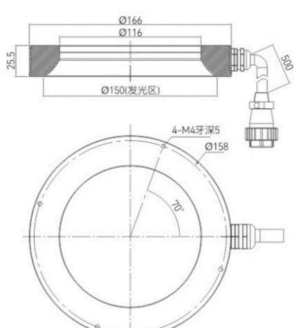
LS-HRM166-8
