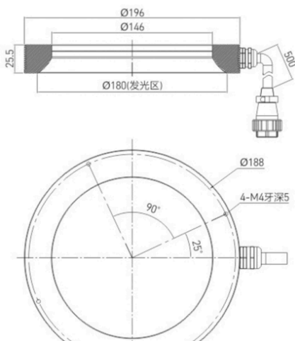
LS-HRM196-4
