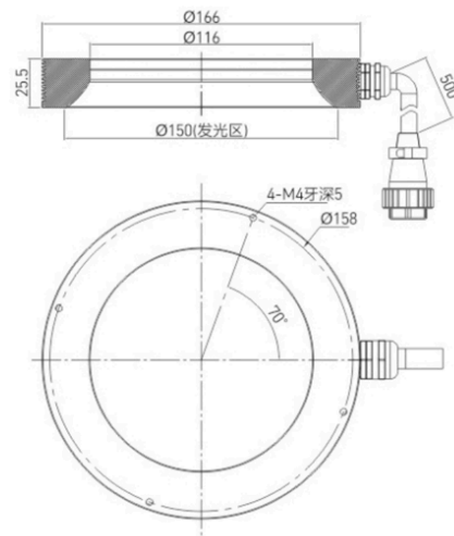
LS-HRM196-8
