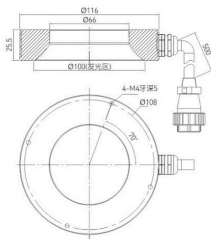
LS-HRM166-8
