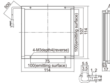
9.LS-2FT100100
