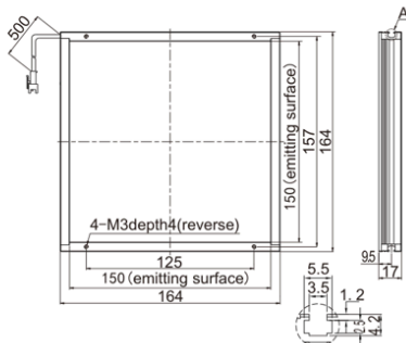
10.LS-2FT150150
