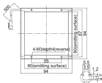
8.LS-2FT8080
