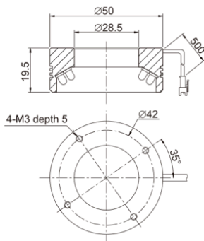
1.LS-RN5060
