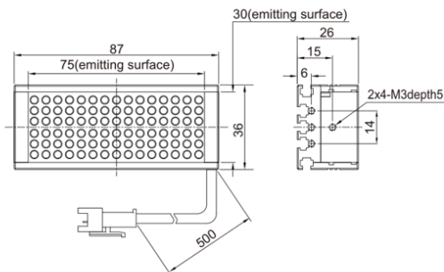
12.LS-2BR7530
