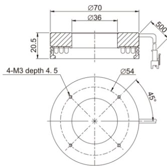
2.LS-RN7090
