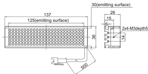
13.LS-2BR12530
