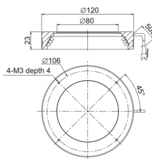
3.LS-RN12030
